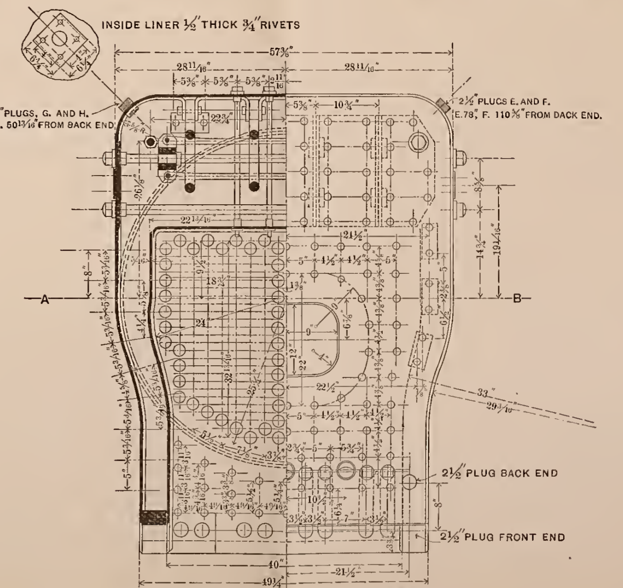
SECTION THROUGH FIRE BOX REAR ELEVATION
